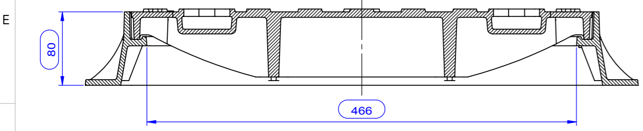
SECTION B-B
